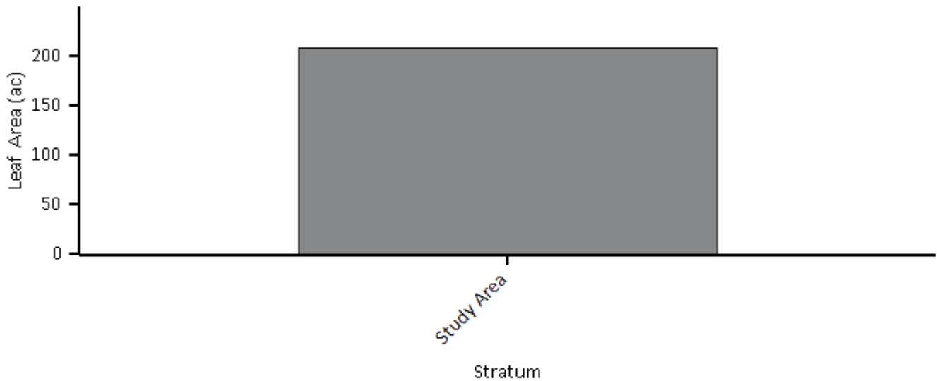
Figure 5. Leaf area by stratum, Holland Twp Inventory
