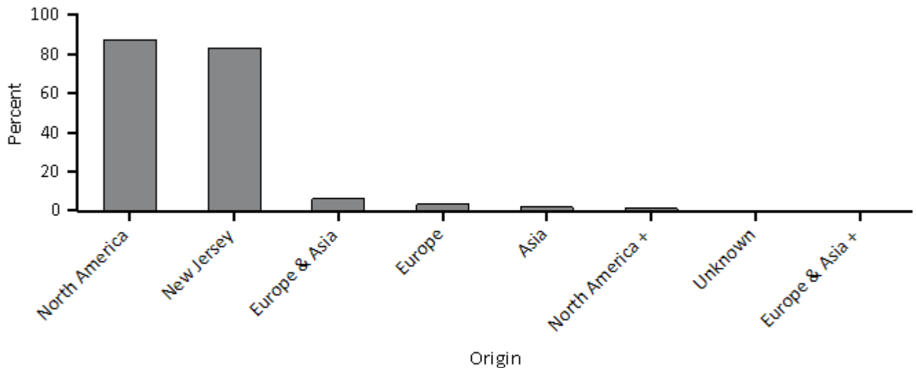
Figure 4. Percent of live tree population by area of native origin, Holland Twp Inventory
