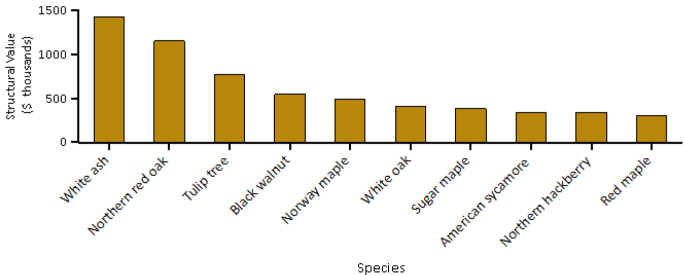
Figure 11. Tree species with the greatest structural value, Holland Twp Inventory
