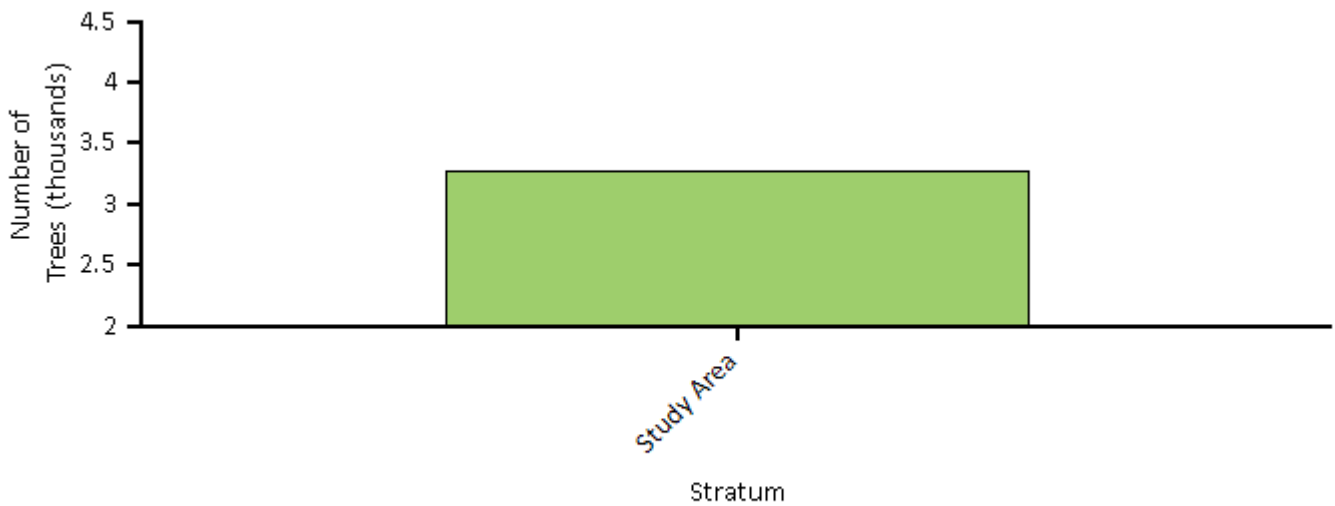
Figure 2. Number of trees in Holland Twp Inventory by stratum
