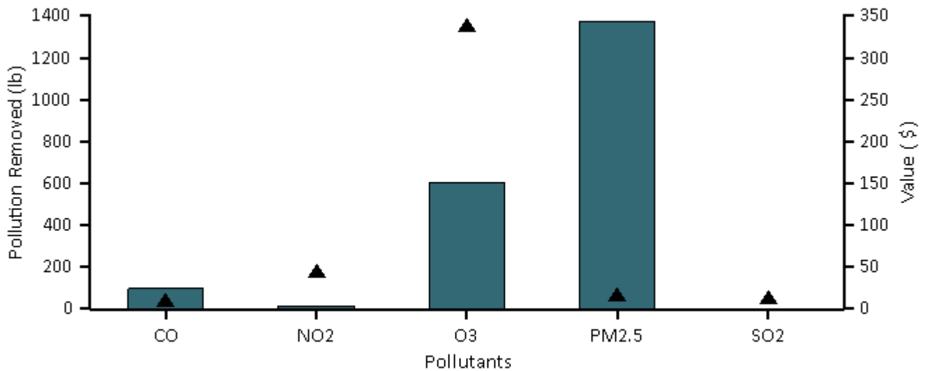
Figure 7. Annual pollution removal (points) and value (bars) by urban trees, Holland Twp Inventory
