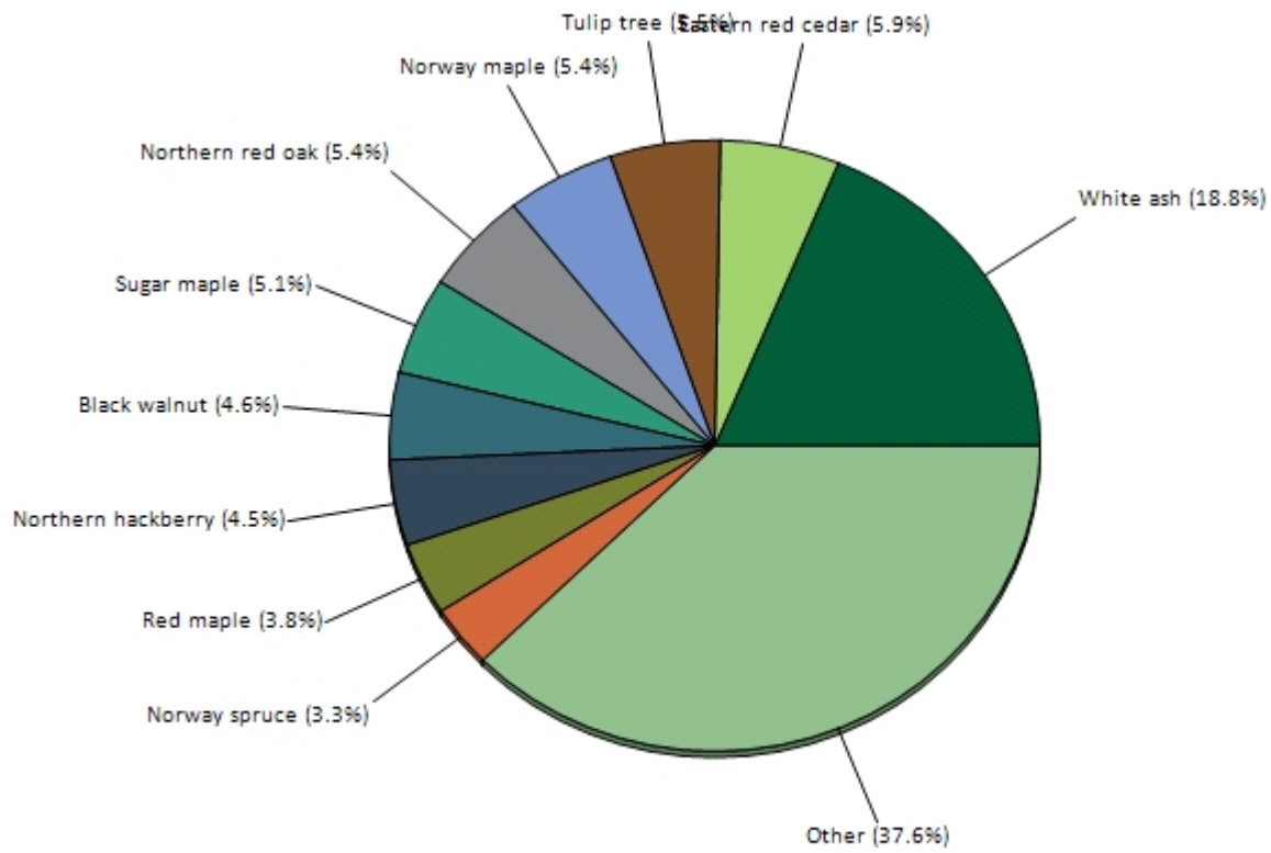
Figure 1. Tree species composition in Holland Twp Inventory
